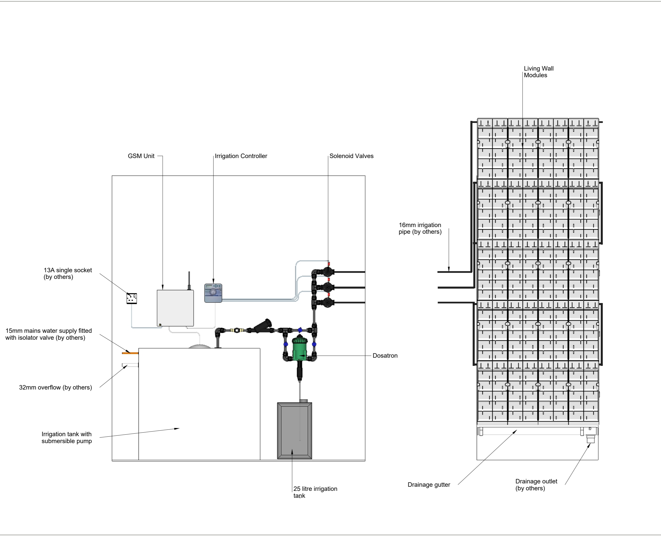
Typical Living Wall Irrigation with Tank Layout
