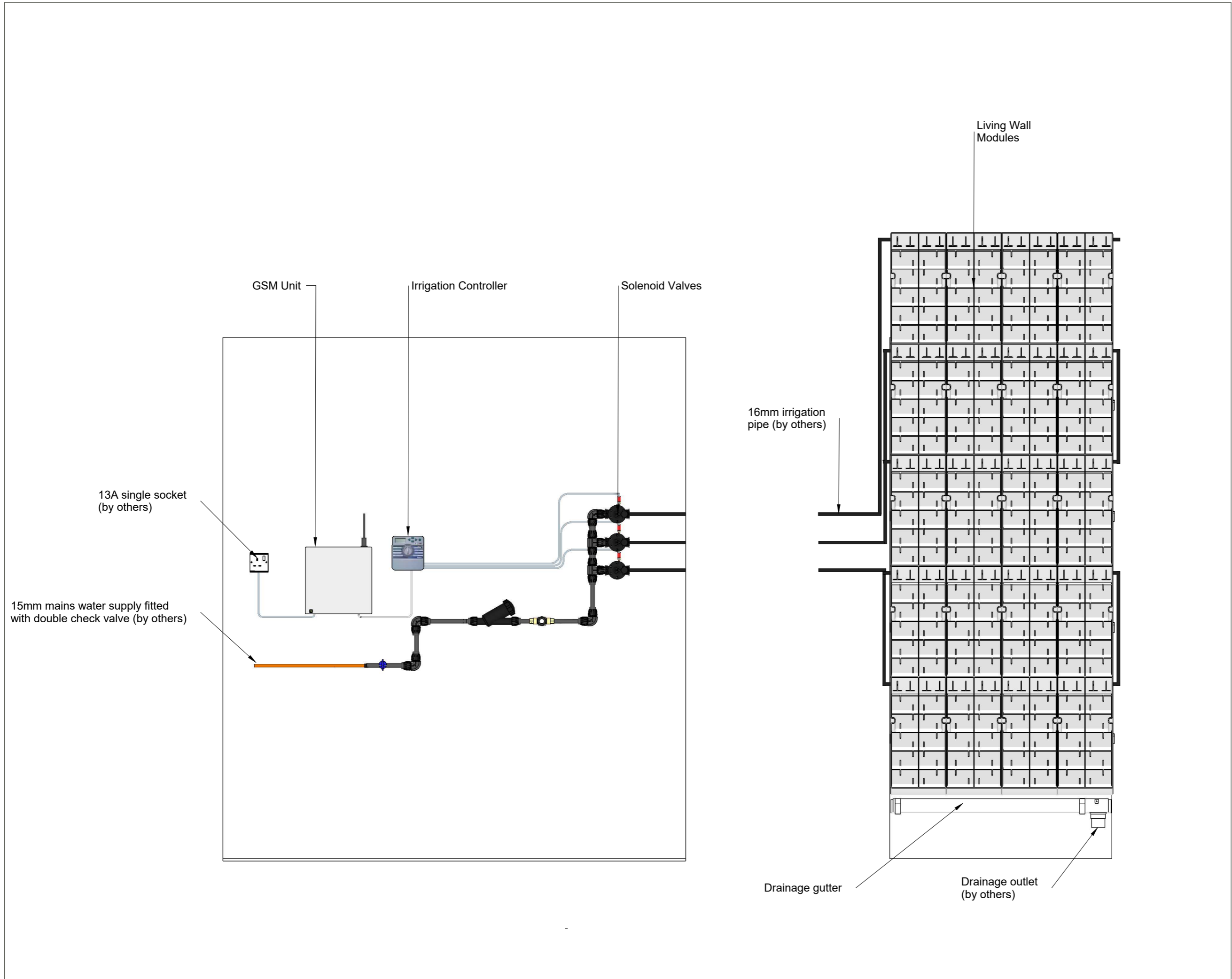
Typical Living Wall Irrigation without Tank Layout
